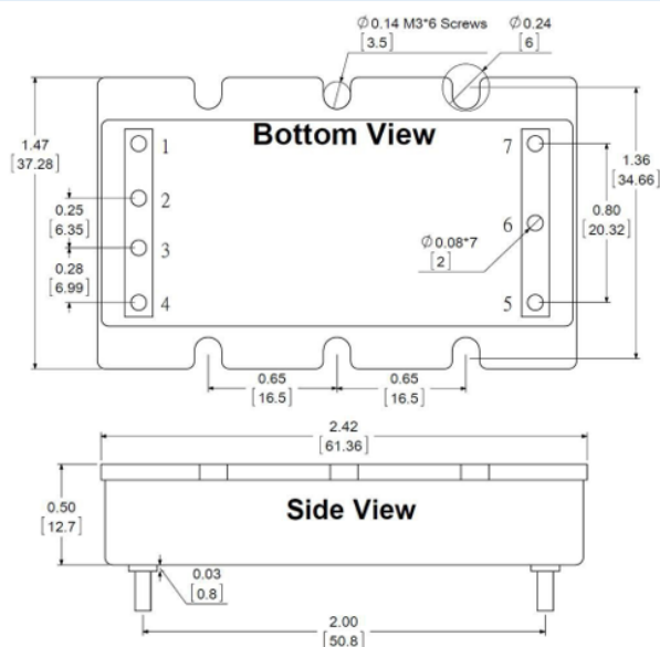
Shape – B (Base Plate with Vicor pinout)
