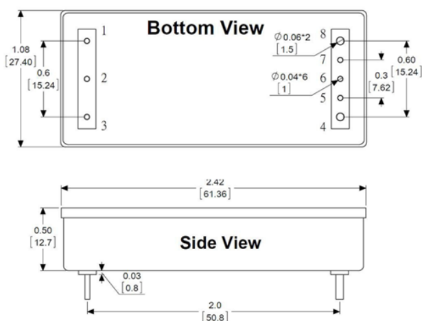
Shape – F (No Flange Base Plate with DOSA pinout)
