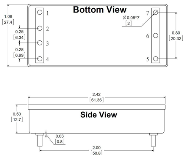
Shape – F (No Flange Base Plate with Vicor pinout)
